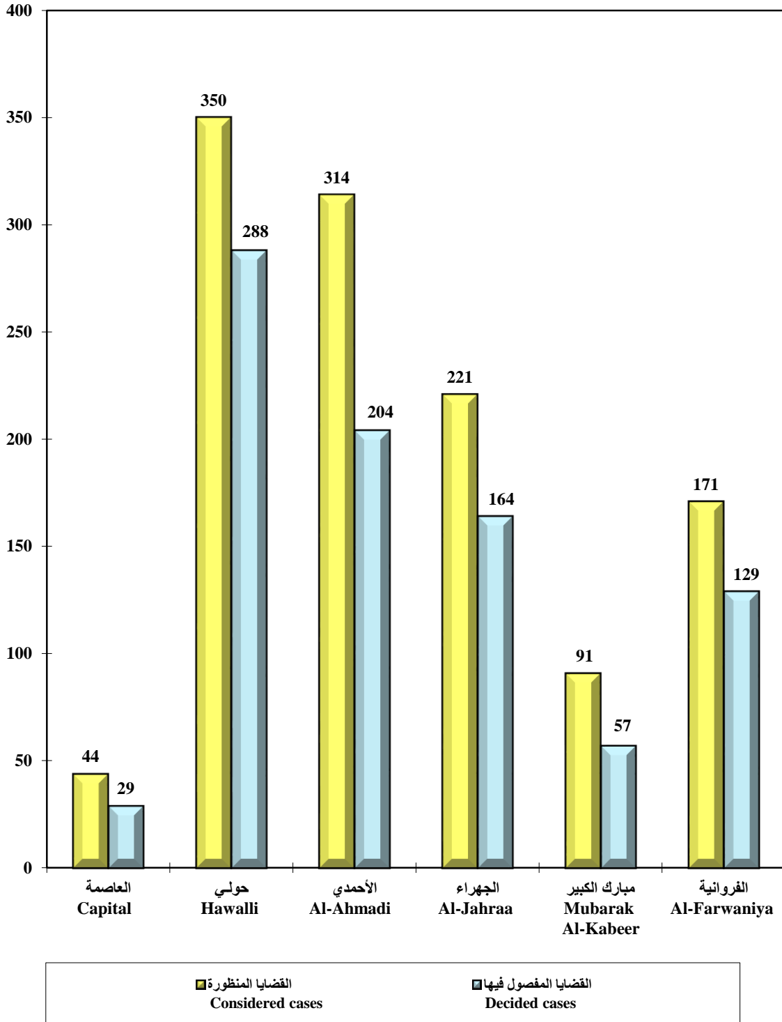
Chart ( 1 ) Number of considered and decided cases in traffic courts during February 2019
